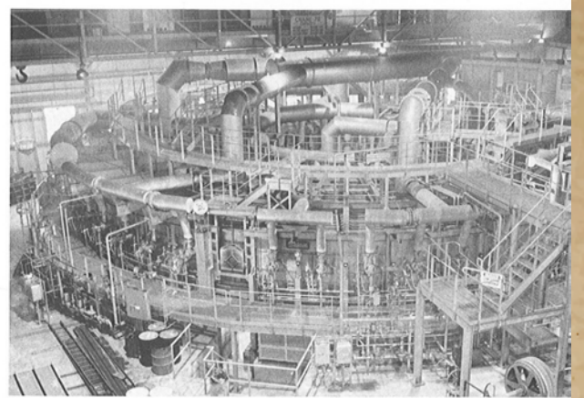
The heart of the new $23.5 million Number 5 Tube Mill is its rotary hearth furnace. The oil or gas-fired furnace is capable of heating steel billets to temperatures in excess of 1027°C. Depending on size, billets are cycled within the furnace from one to three hours until they reach a red-hot stage.
