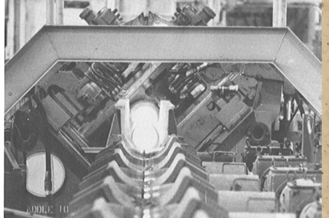
Seamless steel tubing is rolled to precise outside diameter sizes in a 10-stand reducing mill at the new Number 5 Tube Mill. The reducing mill is designed specially to handle a rapid change of tube sizes being rolled at the new facility.
